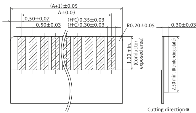
Applicable FPC/FFC dimensions
