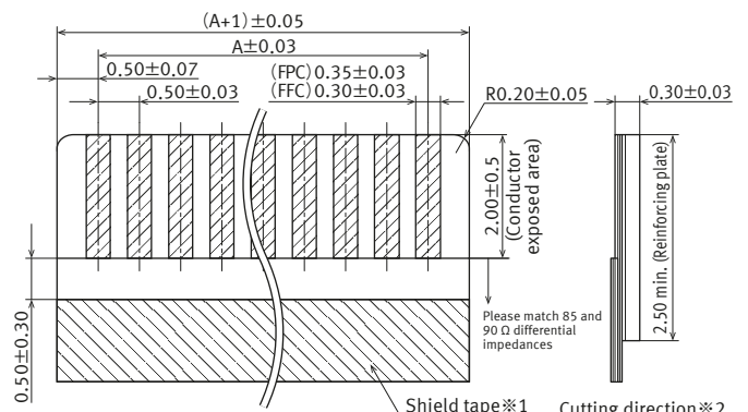
Applicable FPC/FFC dimensions
