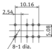
Recommended PC board pattern (BOTTOM VIEW)
