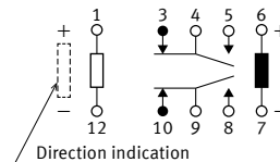
Schematic (BOTTOM VIEW) (Reset) (Operation function LT)
