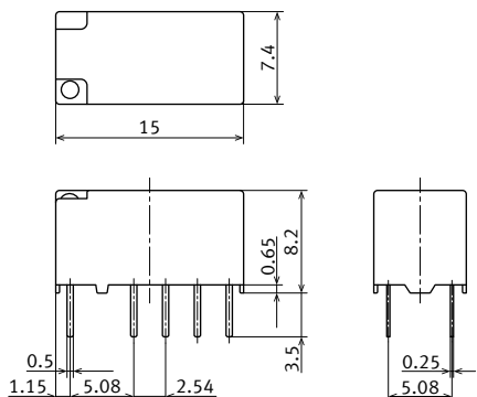
External dimensions
